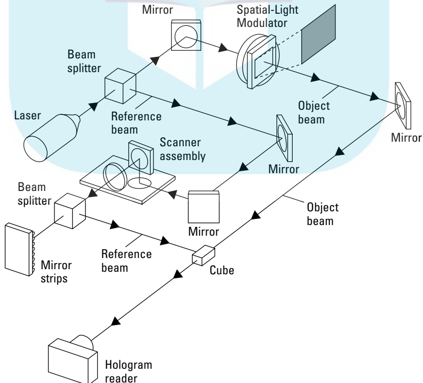
Figure 6-15: Holographic storage layout.
